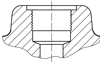
Figure 19 — Machined face suitable for gasket containment if using cylindrical threads
